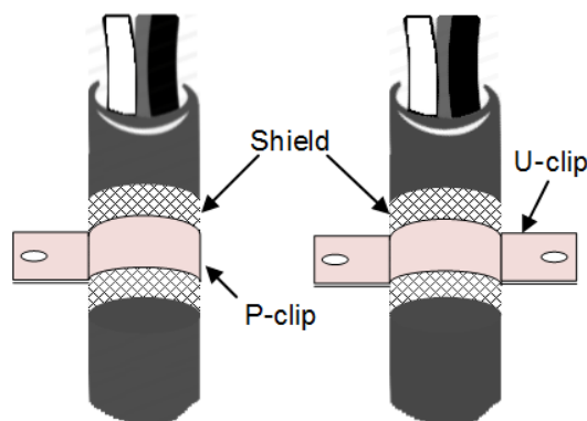
Example of P-clip and U-clip
