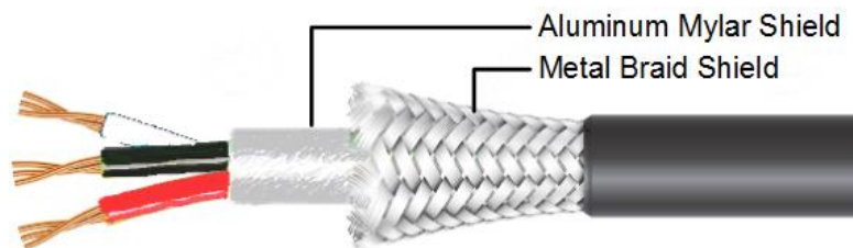
Cable with 2 layer shielding
